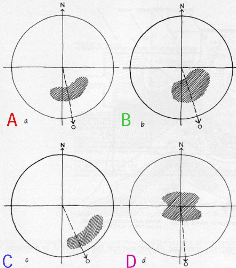
Figure 4.19: Schematic site plans of a hill showing desirable site locations in four climates: (a) cold, (b) temperate, (c) hot arid, and (d) warm humid. (After Olgay, 1963.)
