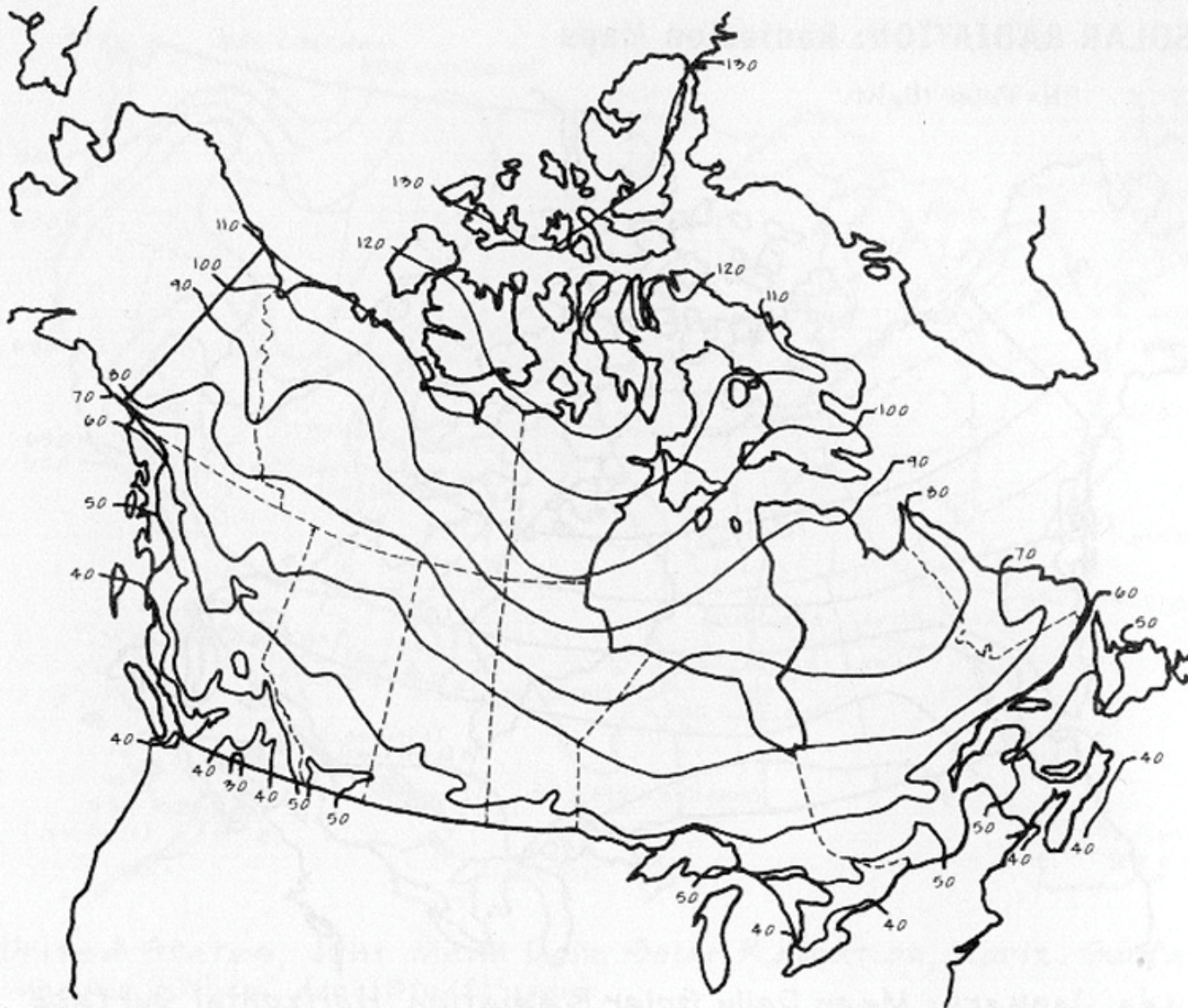
Annual Heating Degree Days for Canada, base 18 °C Source: based on Environment Canada (1988).
