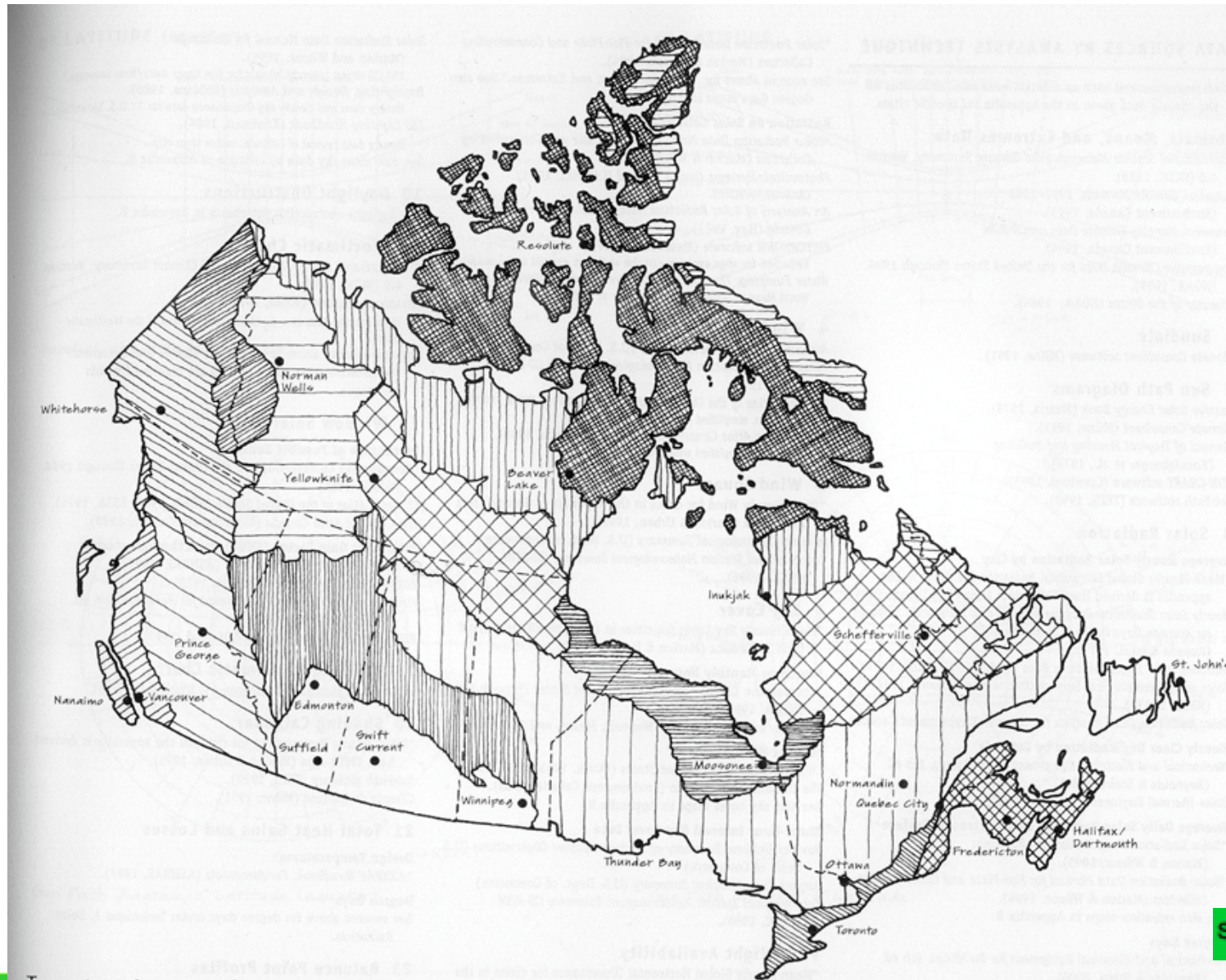
Terrestrial Ecozones of Canada based on Environment Canada (1995).
