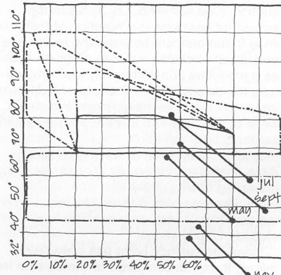
Bioclimatic Chart - Madison
