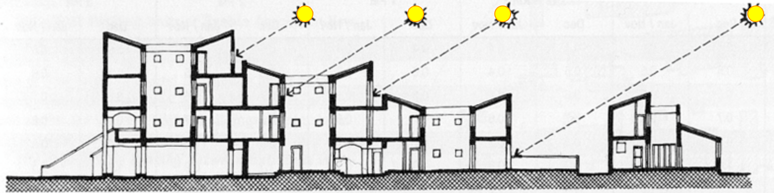
North-South Section, Public Housing Estate, Giudecca Island, Venice, Italy, Gino Valle
