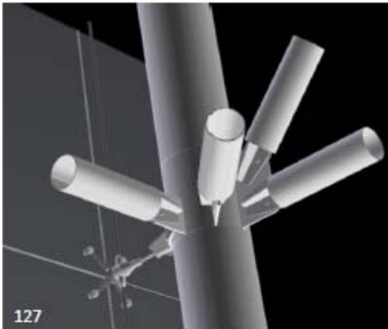
127 3-D modelled detail as can be used to verify connection details through a digital mock-up.
