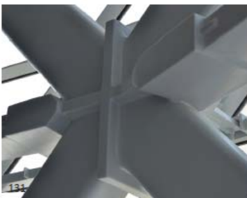
131 This heavy connection in a diagrid uses welding in combination with plates and RHS members to aesthetically handle the large load paths in this node.
