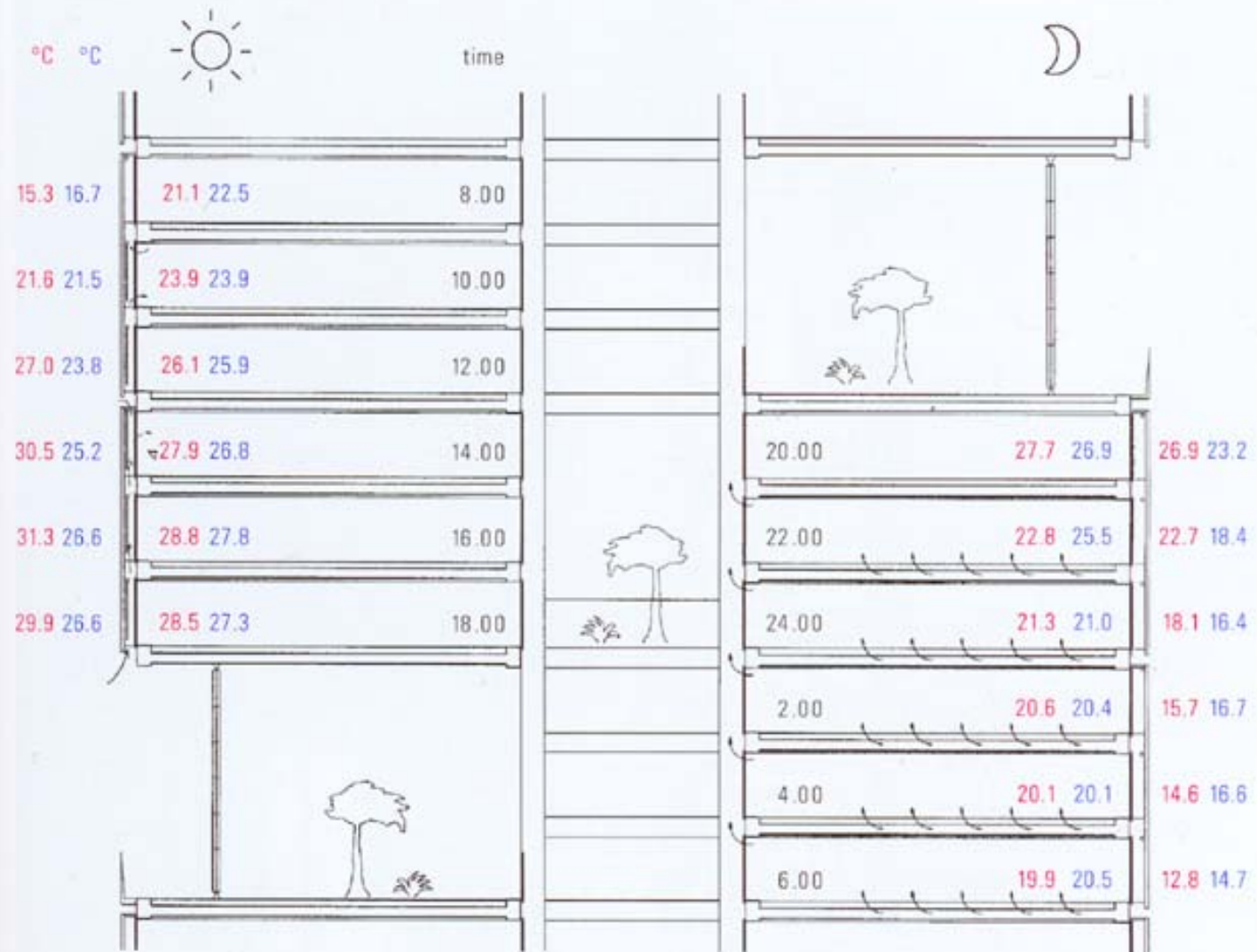
Figure 98.1 Temperature simulations (24 hours) in offices External and room temperatures over the course of one day left column day, right column night
