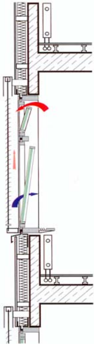
1.1 Comparison of single-skin and double-skin facade construction.
