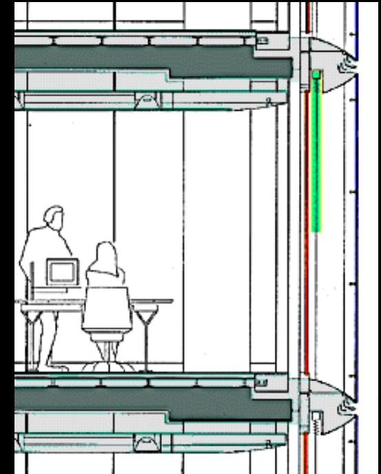
RWE section
