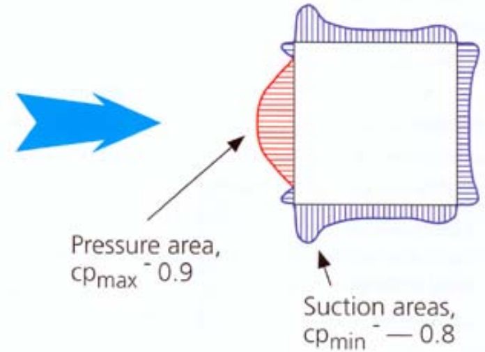
9-3 Far right: qualitative pressure distribution around a high-rise building with a square plan, where the wind direction is at right angles to one side.
