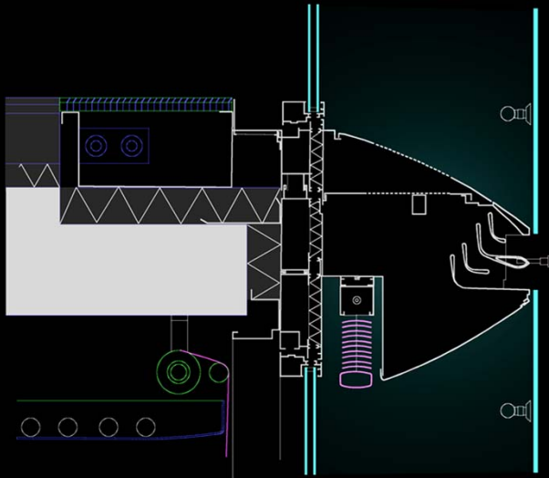
The "fish-mouth" detail
