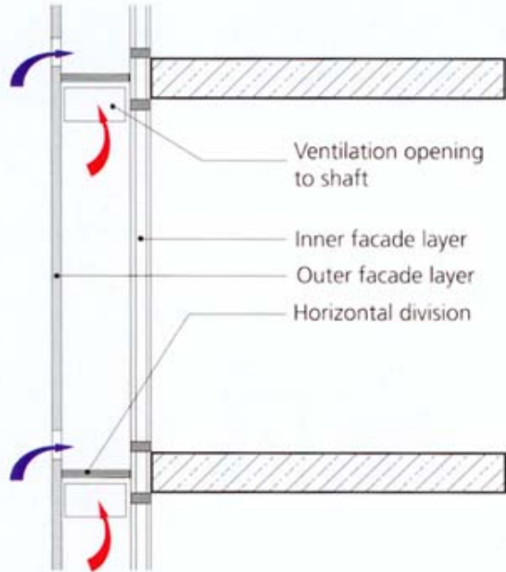
1.9 Section through a shaft-box facade. The arrows indicate the route of the airstream flowing through the box windows into the common ventilation shaft.
