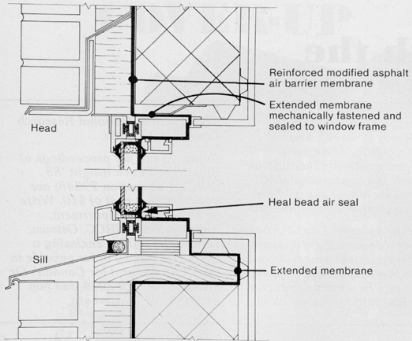
Fig. 1 Commercial Window
