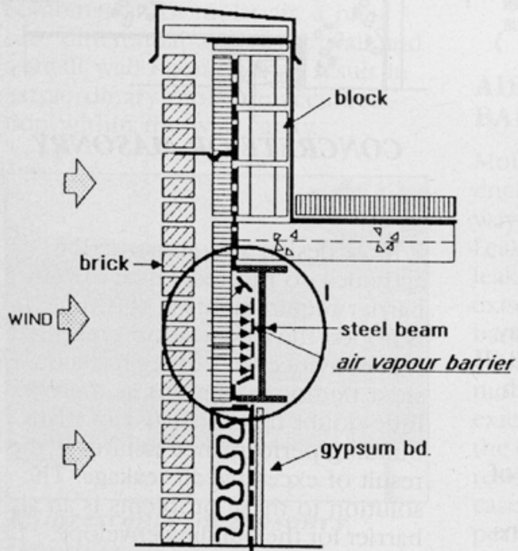
AIR BARRIER RESISTS DISPLACEMENT
