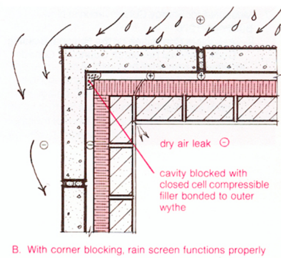
B. With corner blocking, rain screen functions properly
