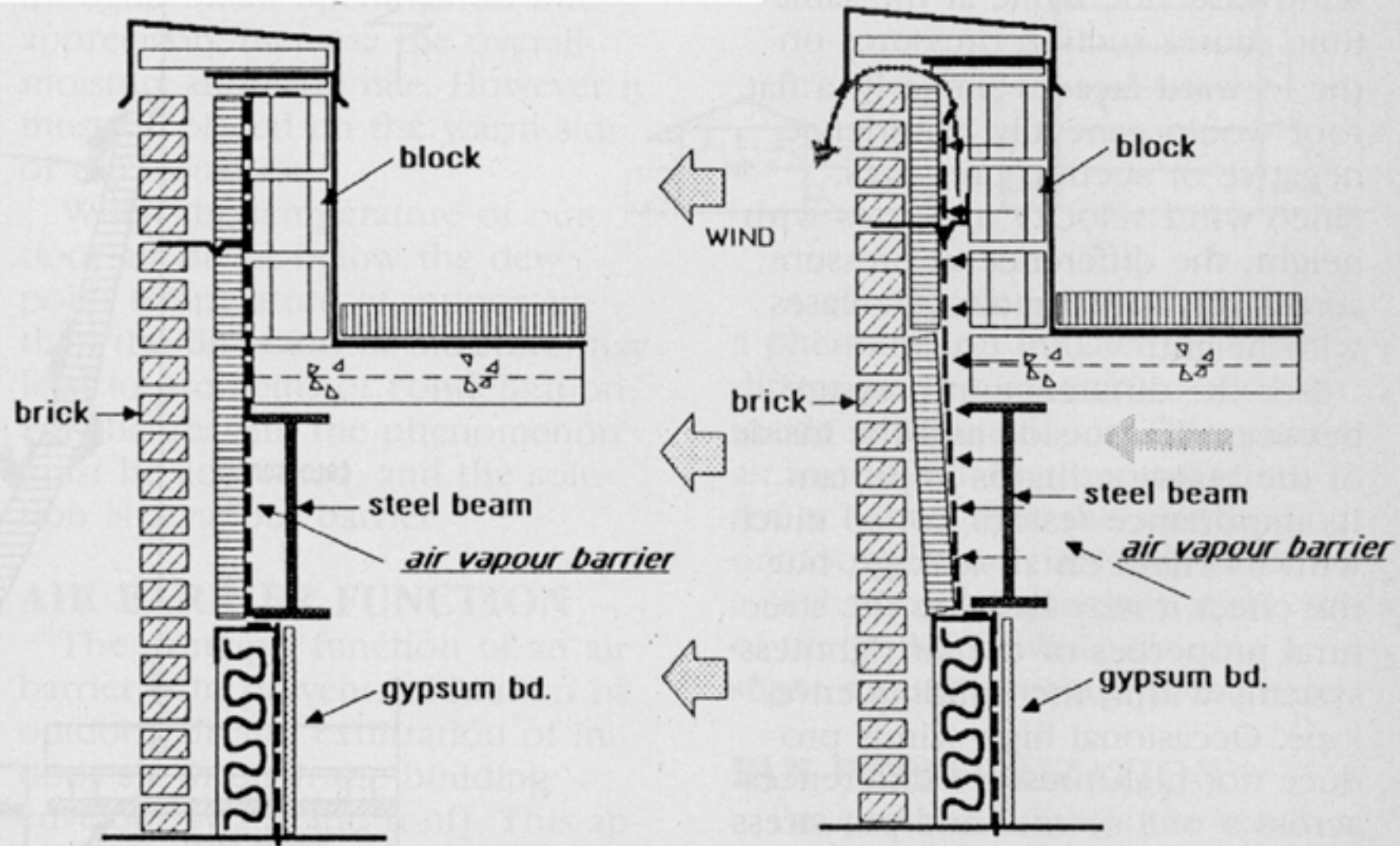
INADEQUATE SUPPORT FOR AIR BARRIER
