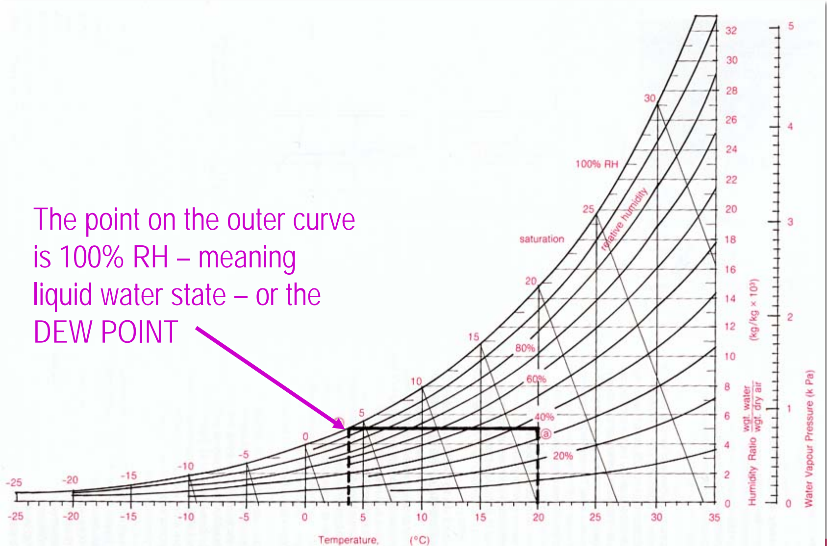
Figure 2.11 Simplified Psychrometric Chart
