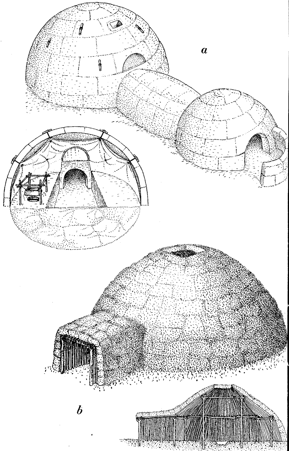
PRIMITIVE DWELLINGS , viewed as engineering structures, extract remarkably high performance from commonplace materials. Eskimo igloo (a) is built from snow blocks 18 inches thick that have insulating value equivalent to two inches of glass fibers. When lined with skins (detail drawing) the temperature of the interior can be raised to 40 degrees F. without melting the dome. Summer house of Nunamiut Eskimos (b) follows igloo plan,
