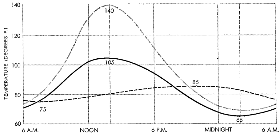
ADOBE HOUSE TEMPERATURES compare favorably with those obtainable in modern air-conditioned homes. Moreover, the solar heat trapped by the roof slab in the daytime keeps the interior warm through the chill night.
