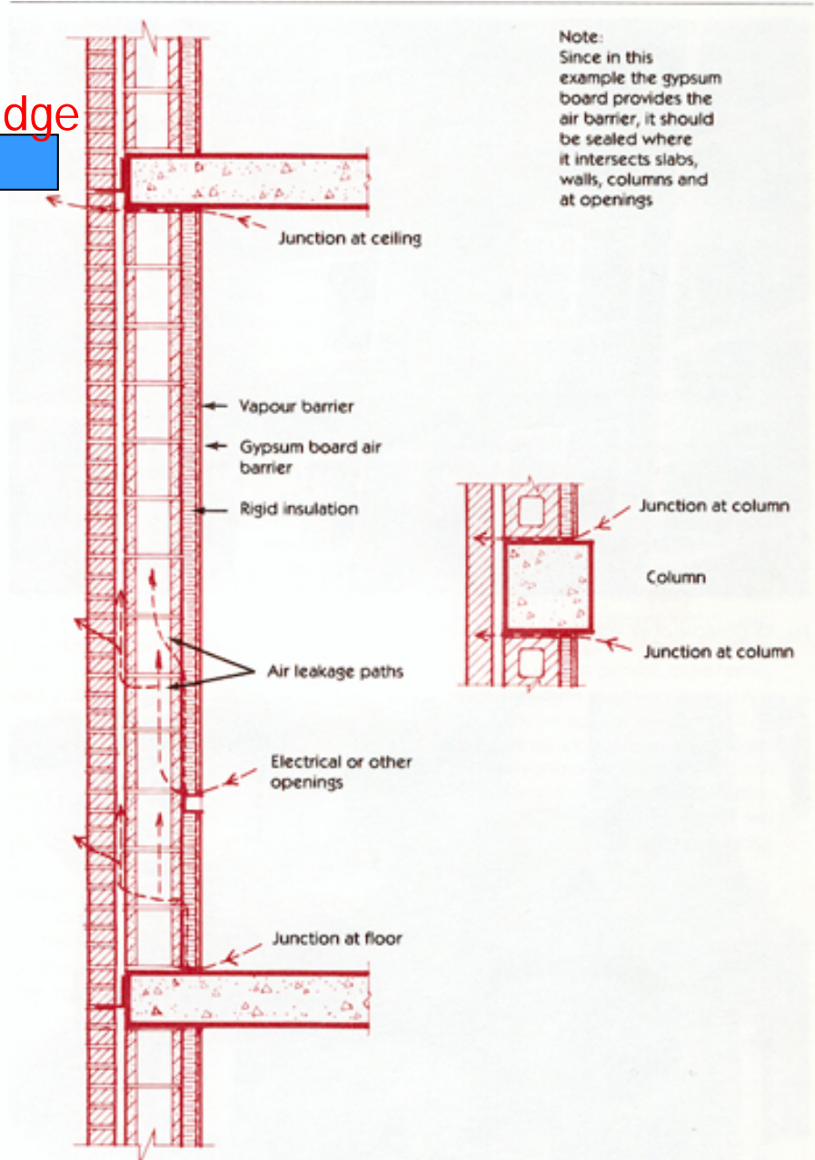
Fig. 17 Air leakage paths in brick veneer on concrete block backup to be taped or otherwise sealed (ties, flashings and weepholes not shown)
