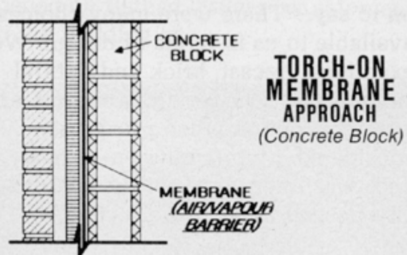
Fig. 7 & 8: Applied Membrane Air Barriers
